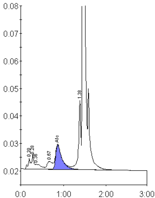
Peak table - ID: 10539128
